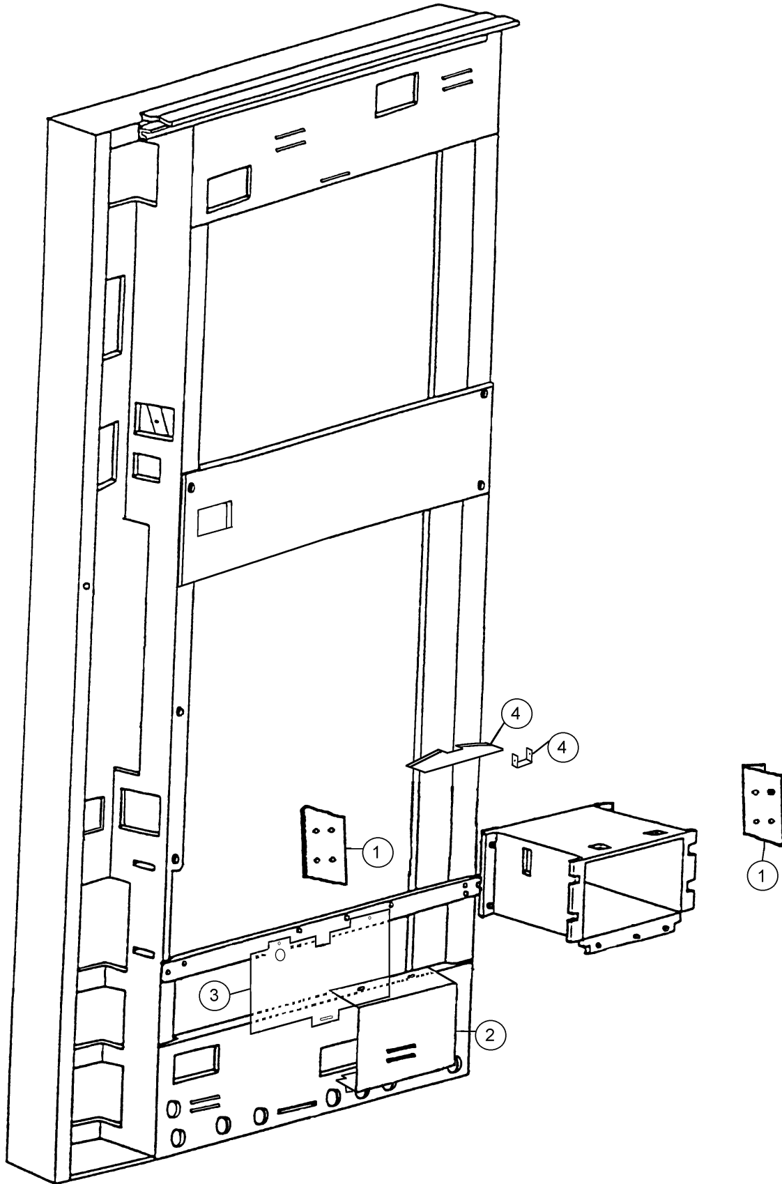
FIGURE 1 MAIN DOOR ASSEMBLY BACK VIEW
