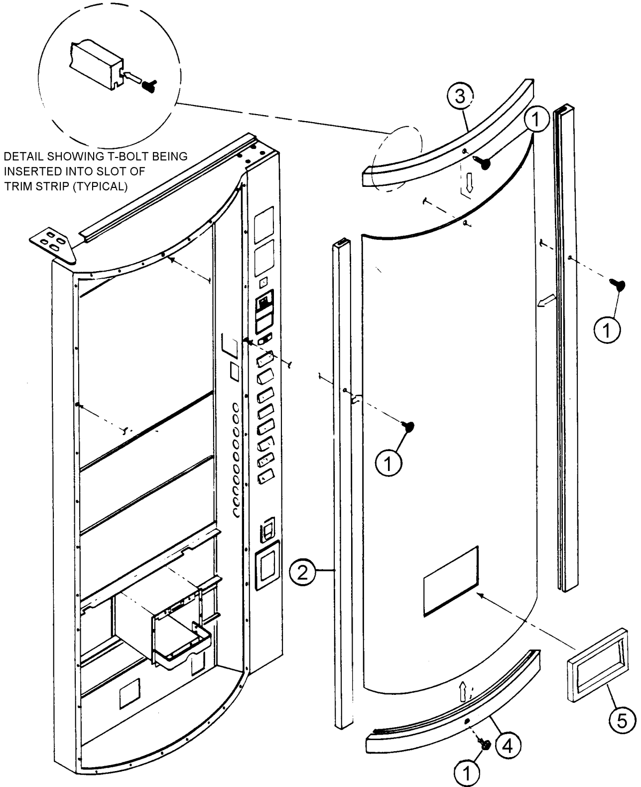
FIGURE 2 MAIN DOOR ASSEMBLY FRONT VIEW
